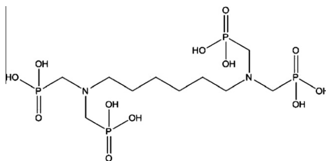
Figure 1 Structure of hexa methylene diamine tetra methyl-phosphonic acid (HMDTMP).
