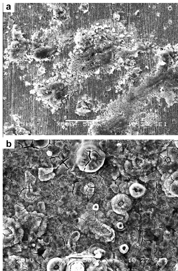
Figure 6 SEM micrographs of samples after immersion in 0.5 M HCl (a) without (b) with 4 \times 10^{-3} M HMDTMP.
