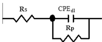
Figure 5 Equivalent circuit used to fit the EIS data of carbon steel in 0.5 M HCl in the presence and absence of HMDTMP.
