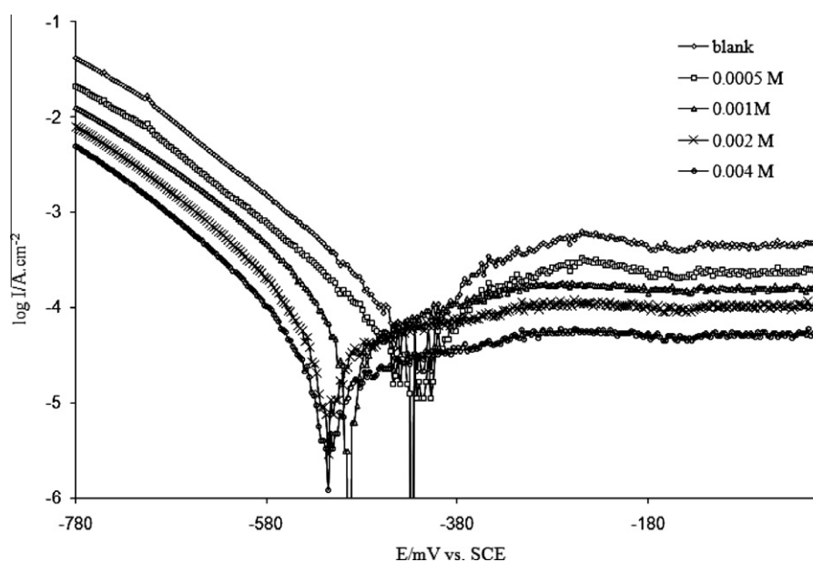
Figure 2 Potentiodynamic polarization curves for mild steel in 0.5 M HCl containing different concentrations of HMDTMP.
