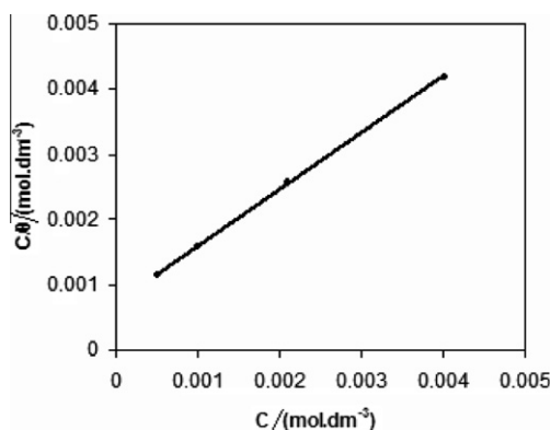
Figure 3 Langmuir adsorption isotherm model of HMDTMP on the carbon steel surface at 298 K.
