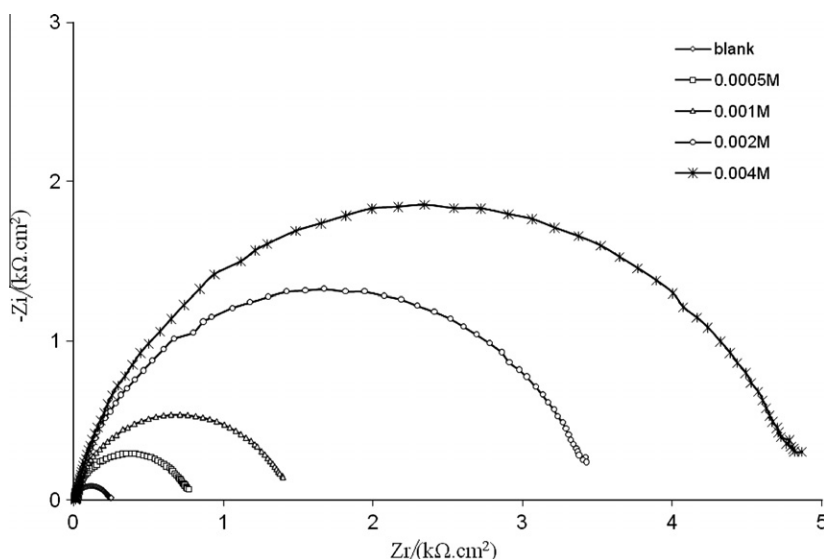
Figure 4 Nyquist plot for MS in 0.5 M HCl in the presence and absence of different concentrations of HMDTMP.
